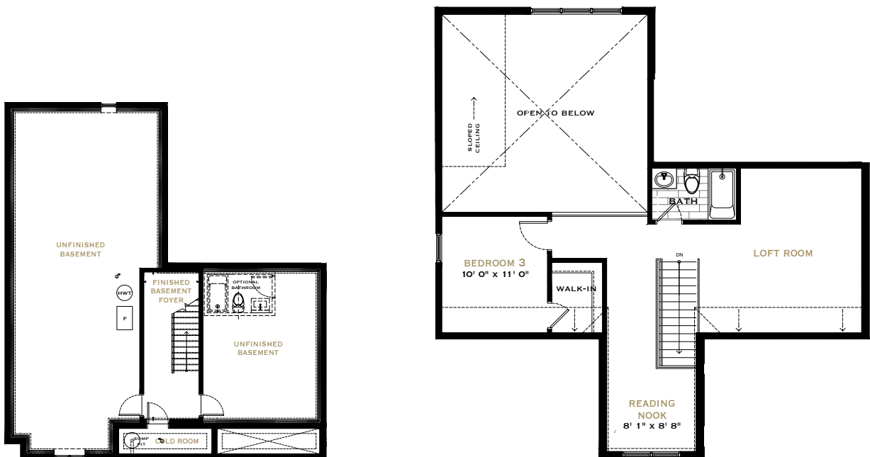
BASEMENT
